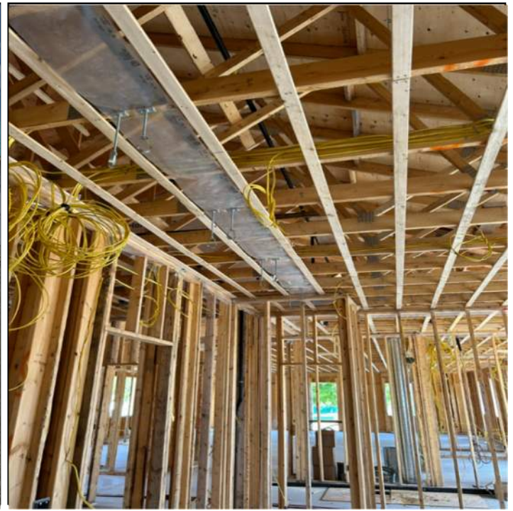
Progress – Interior framing / rough-ins
